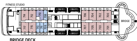
BRIDGE DECK
